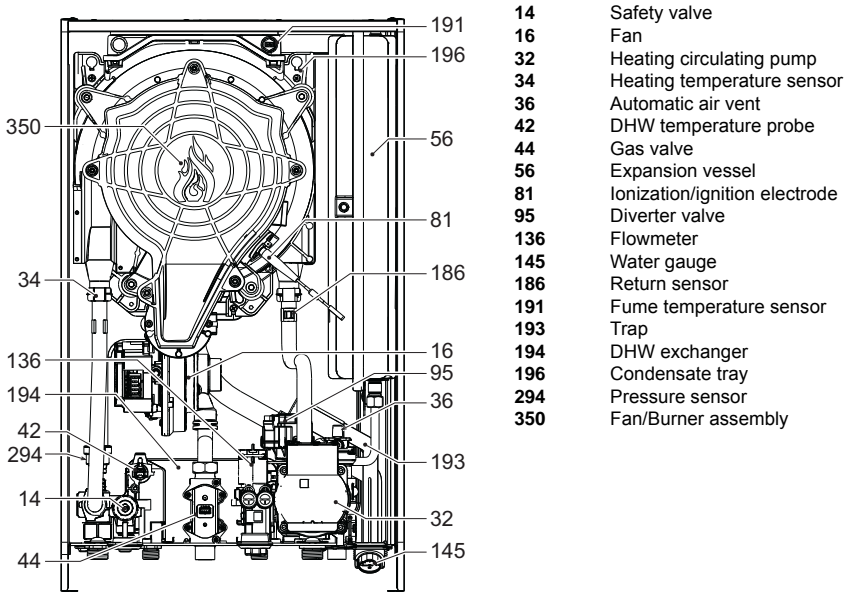
fig. 62- General view
