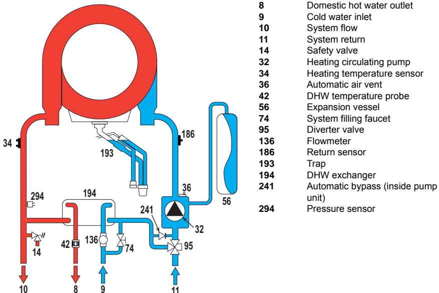
fig. 63- Hydraulic circuit
